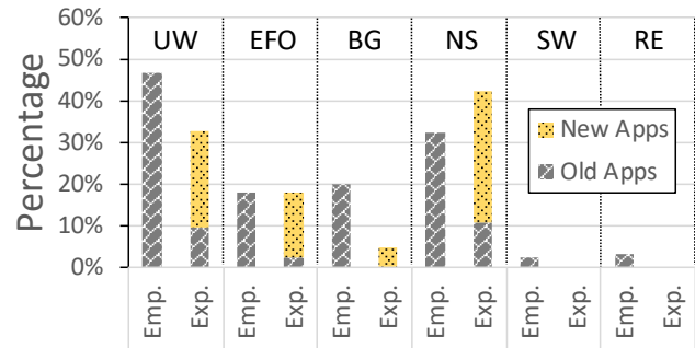
Figure 7: Issue causes in empirical study and experiment.
